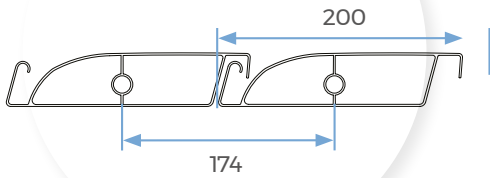
1 LAMELLA
